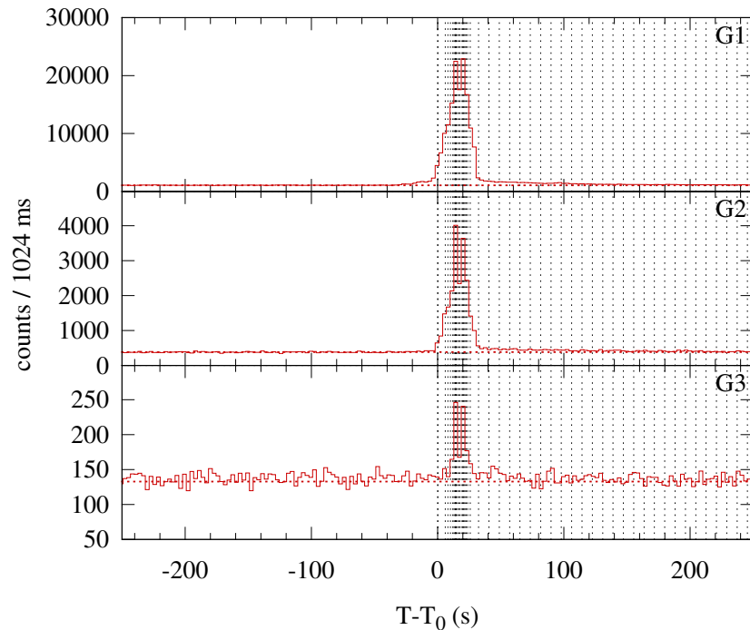
Konus-WIND S2 SOL2014-10-21T13:36 (M1.2) T_0 = 49017.346 s UT (13:36:57.346)
