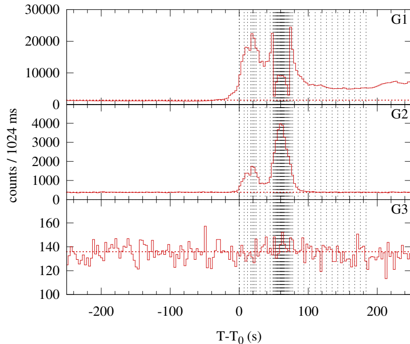
Konus-WIND S2 SOL2014-10-22T01:38 (M8.7) T 0 = 5895.841 s UT (01:38:15.841)
