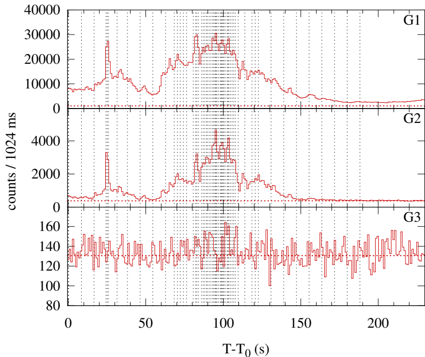
Konus-WIND S2 SOL2014-10-24T07:40 (M4.0) T 0 = 27621.997 s UT (07:40:21.997)
