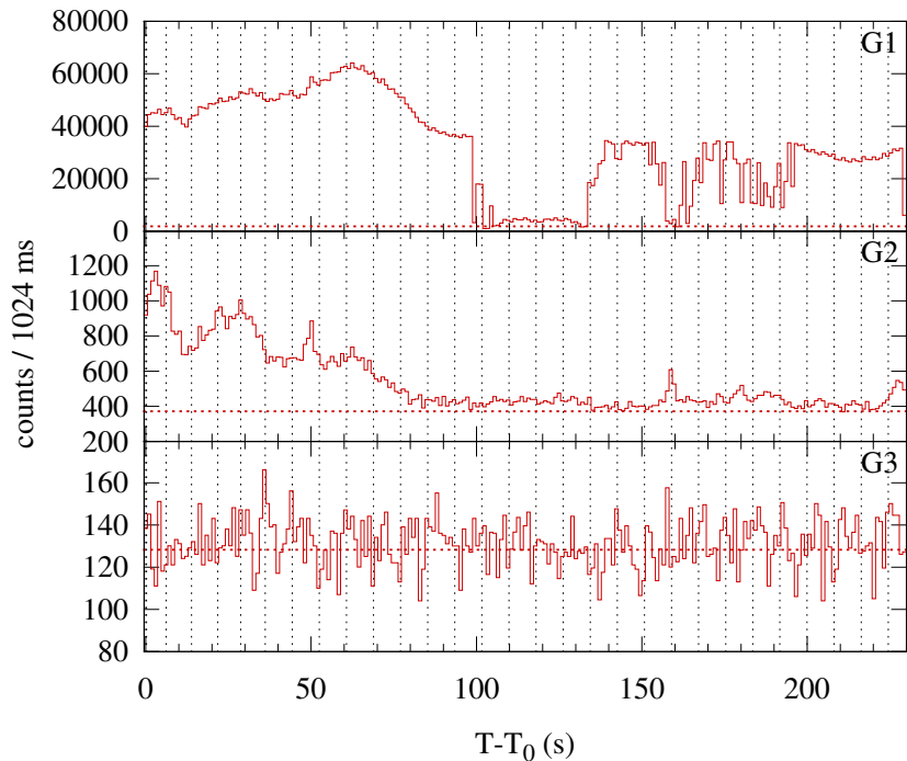
Konus-WIND S2 SOL2014-10-26T10:42 (X2.0) T_0 = 38574.688 s UT (10:42:54.688)
