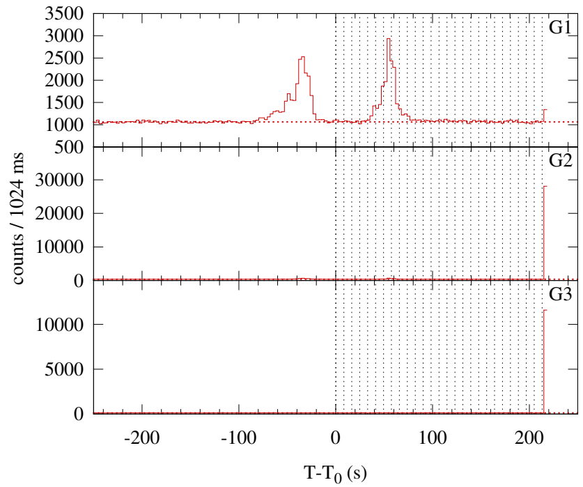
Konus-WIND S2 SOL2014-11-07T16:37 (C7.0) T 0 = 59827.335 s UT (16:37:07.335)
