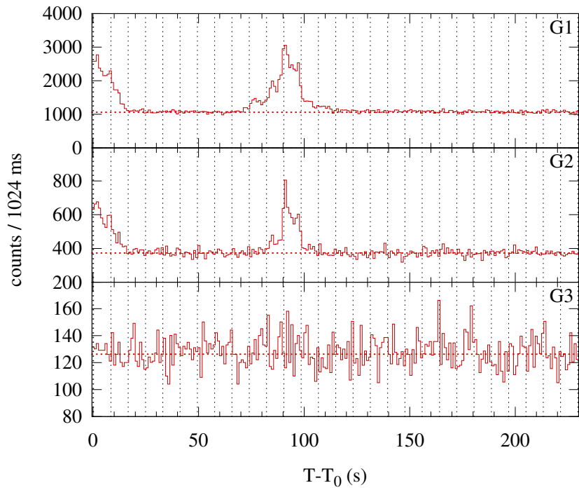
Konus-WIND S2 SOL2014-11-07T16:37 (C7.0) T 0 = 59827.335 s UT (16:37:07.335)
