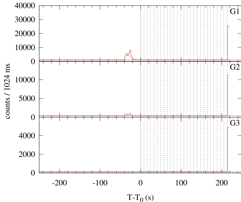
Konus-WIND S2 SOL2014-11-10T02:21 (C7.6) T 0 = 8500.790 s UT (02:21:40.790)
