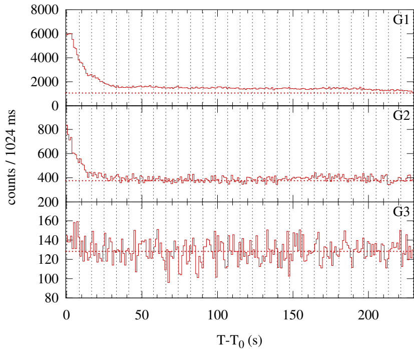
Konus-WIND S2 SOL2014-11-15T20:43 (M3.7) T_0 = 74582.734 s UT (20:43:02.734)
