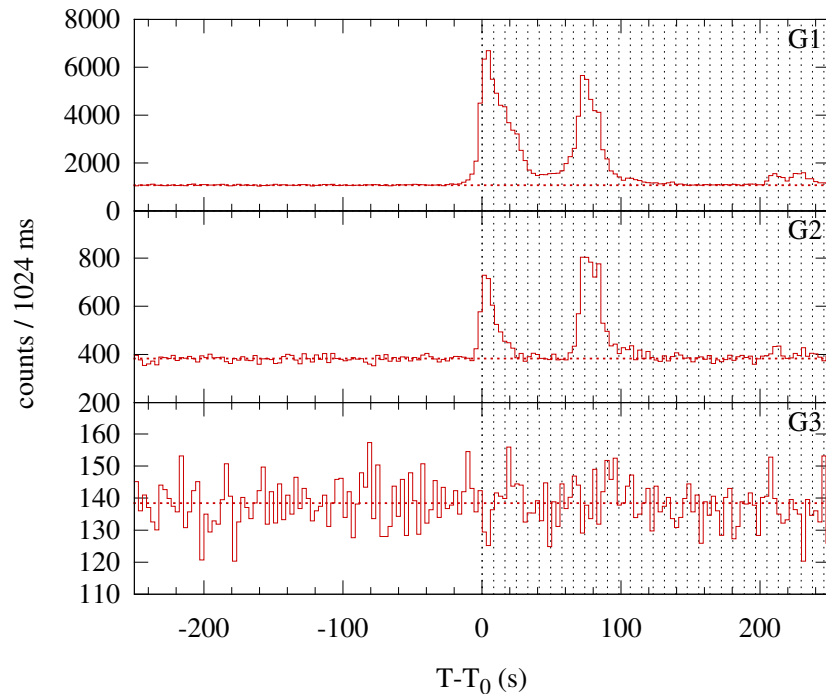
Konus-WIND S2 SOL2014-11-29T08:19 (C6.7) T 0 = 29960.744 s UT (08:19:20.744)
