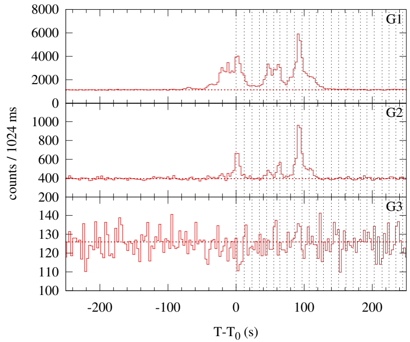
Konus-WIND S2 SOL2015-01-03T09:45 (M1.1) T 0 = 35117.758 s UT (09:45:17.758)
