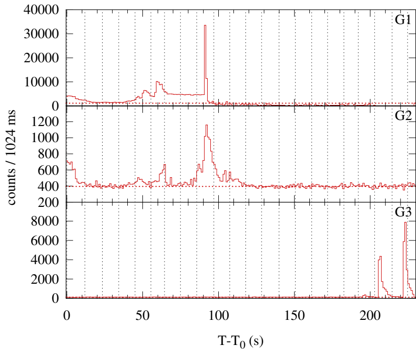
Konus-WIND S2 SOL2015-01-03T09:45 (M1.1) T 0 = 35117.758 s UT (09:45:17.758)
