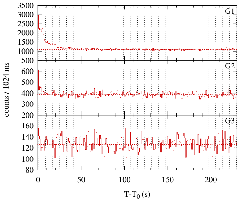
Konus-WIND S2 SOL2015-03-09T00:14 (C3.0) T 0 = 862.885 s UT (00:14:22.885)
