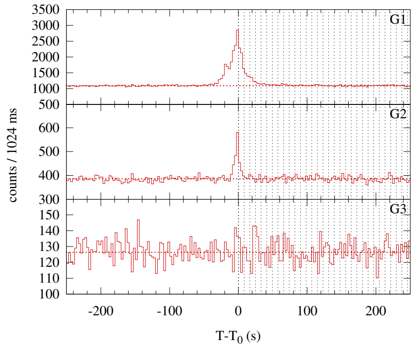
Konus-WIND S2 SOL2015-03-09T00:14 (C3.0) T 0 = 862.885 s UT (00:14:22.885)
