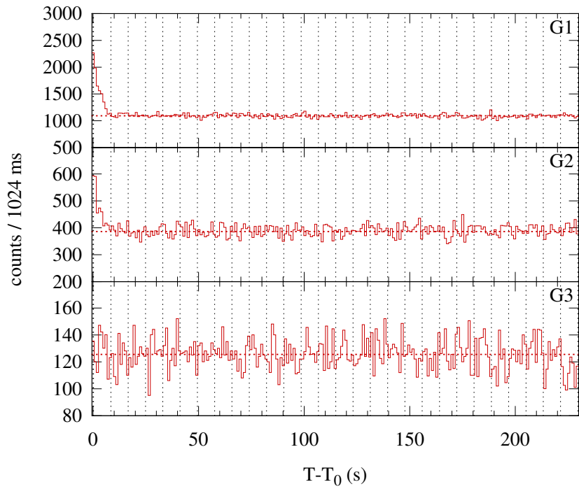
Konus-WIND S2 SOL2015-03-10T06:32 (C1.4) T_0 = 23527.547 s UT (06:32:07.547)
