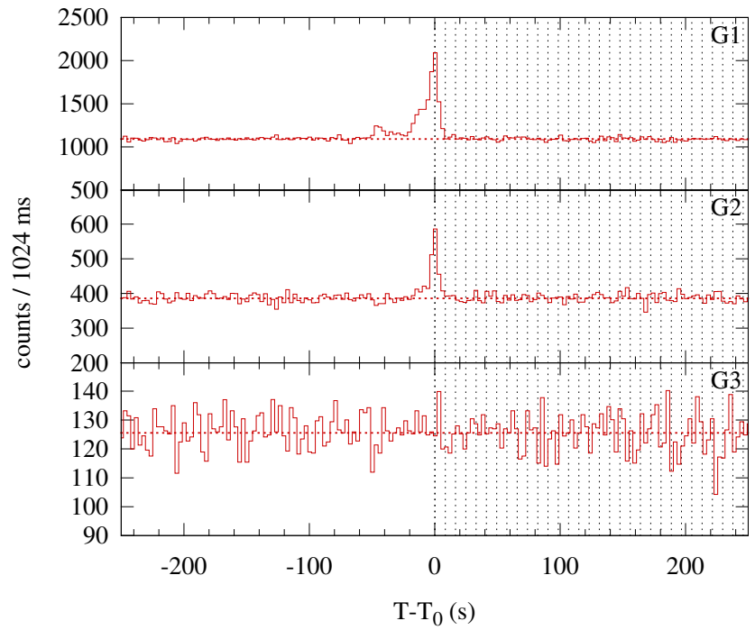
Konus-WIND S2 SOL2015-03-10T06:32 (C1.4) T_0 = 23527.547 s UT (06:32:07.547)
