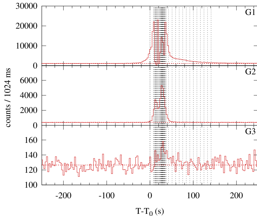
Konus-WIND S2 SOL2015-03-10T23:59 (M2.9) T 0 = 86391.1 s UT (23:59:51.1)
