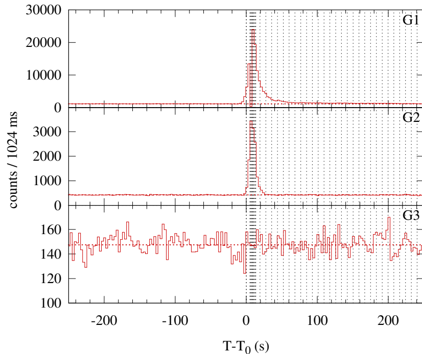
Konus-WIND S2 SOL2015-03-15T09:37 (M1.0) T 0 = 34620.111 s UT (09:37:00.111)
