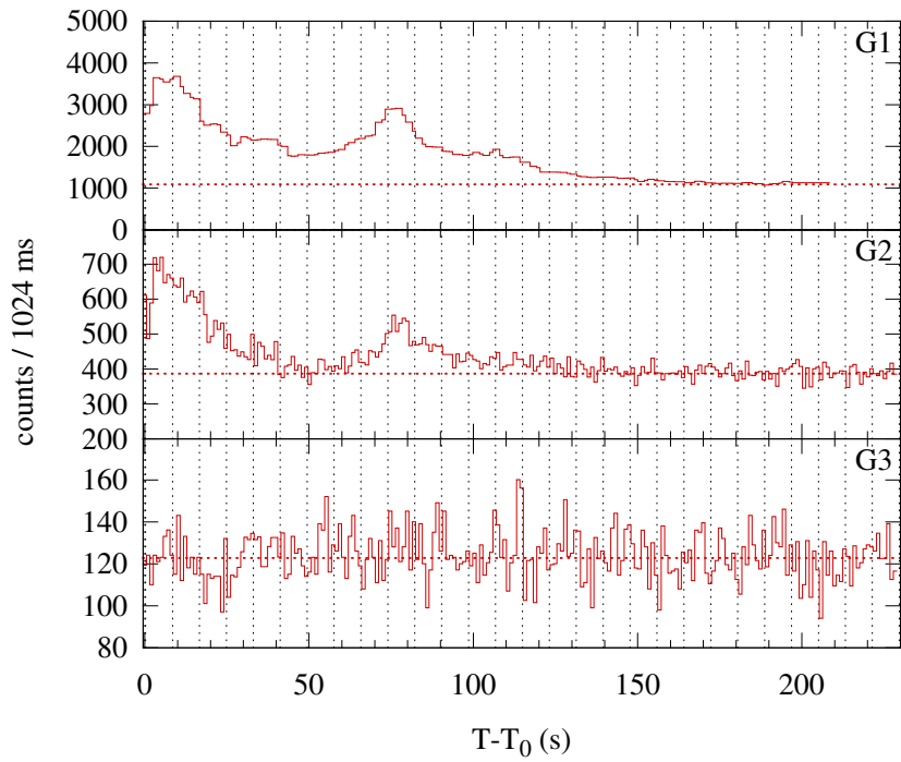
Konus-WIND S2 SOL2015-04-08T14:40 (M1.4) T_0 = 52837.845 s UT (14:40:37.845)
