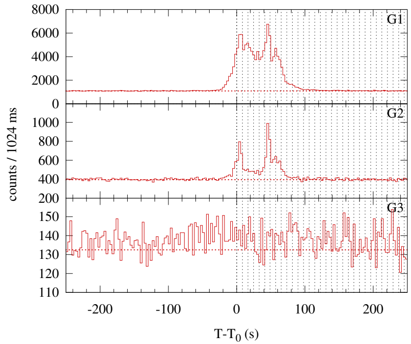
Konus-WIND S2 SOL2015-05-06T11:47 (M1.9) T 0 = 42473.814 s UT (11:47:53.814)
