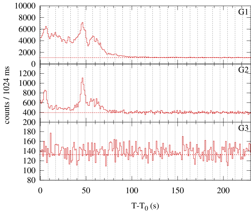
Konus-WIND S2 SOL2015-05-06T11:47 (M1.9) T 0 = 42473.814 s UT (11:47:53.814)
