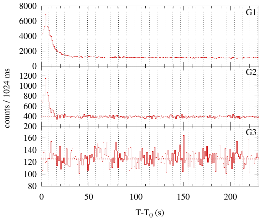
Konus-WIND S2 SOL2015-05-08T04:06 (C5.5) T 0 = 14768.360 s UT (04:06:08.360)
