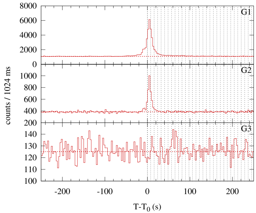
Konus-WIND S2 SOL2015-05-08T04:06 (C5.5) T 0 = 14768.360 s UT (04:06:08.360)
