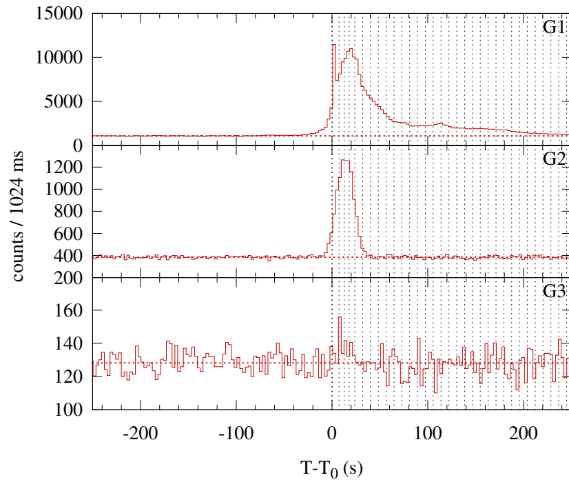
Konus-WIND S2 SOL2015-06-14T00:55 (M2.0) T_0 = 3304.965 s UT (00:55:04.965)
