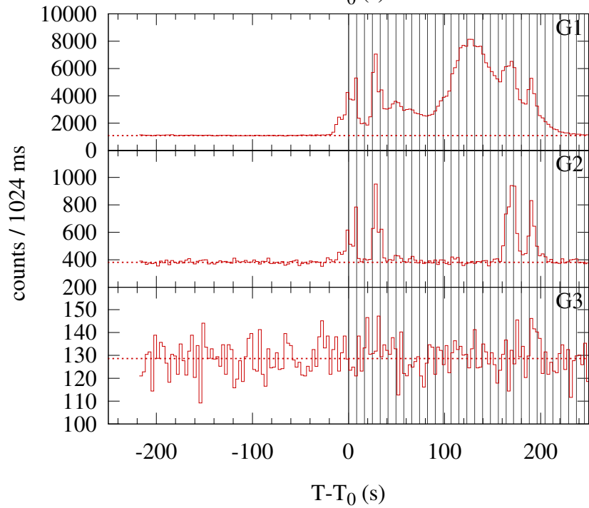
Konus-WIND S2 SOL2015-08-24T07:30 (M5.6) T 0 = 27030.85 s UT (07:30:30.85)
