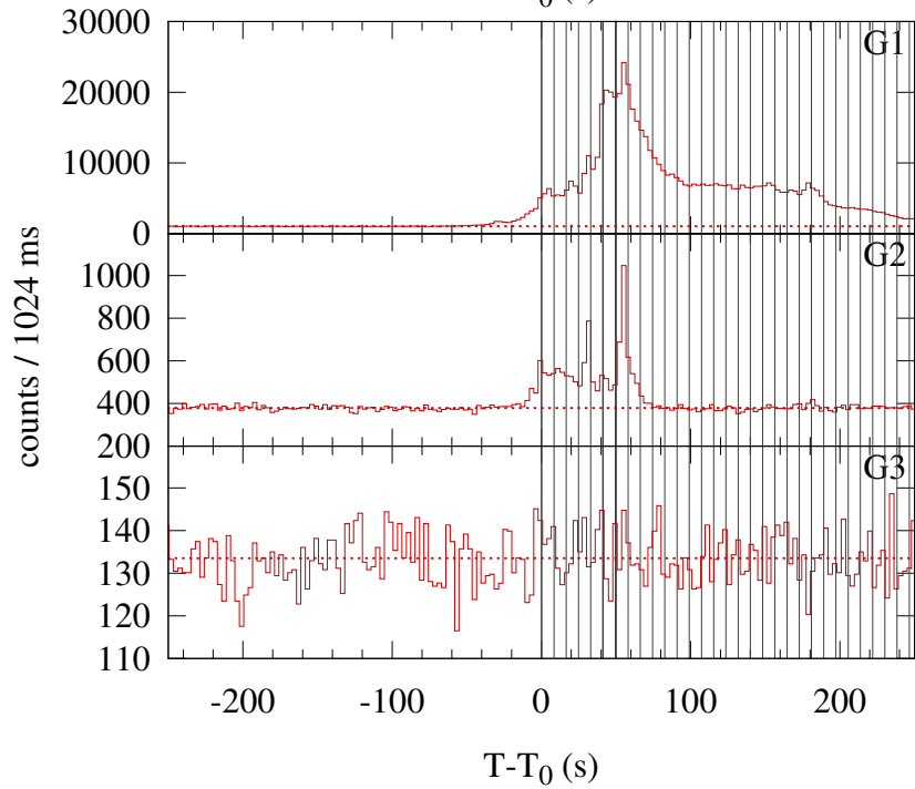
Konus-WIND S2 SOL2015-09-28T14:54 (M7.6) T 0 = 53697.238 s UT (14:54:57.238)
