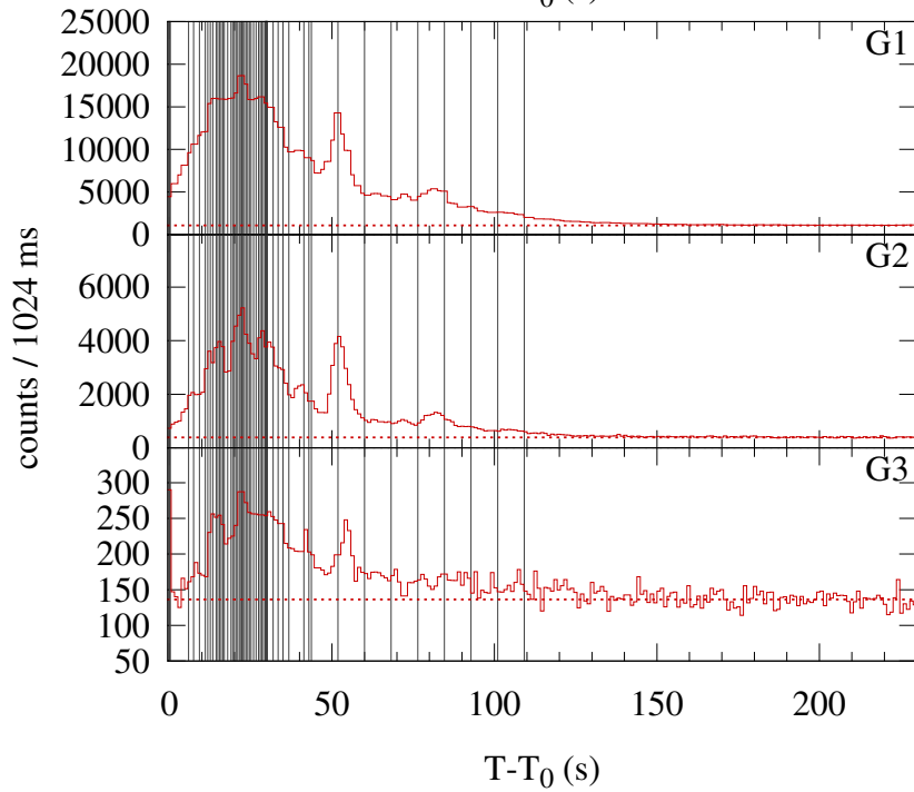
Konus-WIND S2 SOL2015-11-04T03:23 (M1.9) T_0 = 12211.938 s UT (03:23:31.938)
