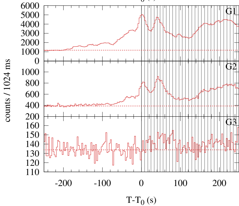
Konus-WIND S2 SOL2015-11-09T13:02 (M3.9) T_0 = 46936.791 s UT (13:02:16.791)
