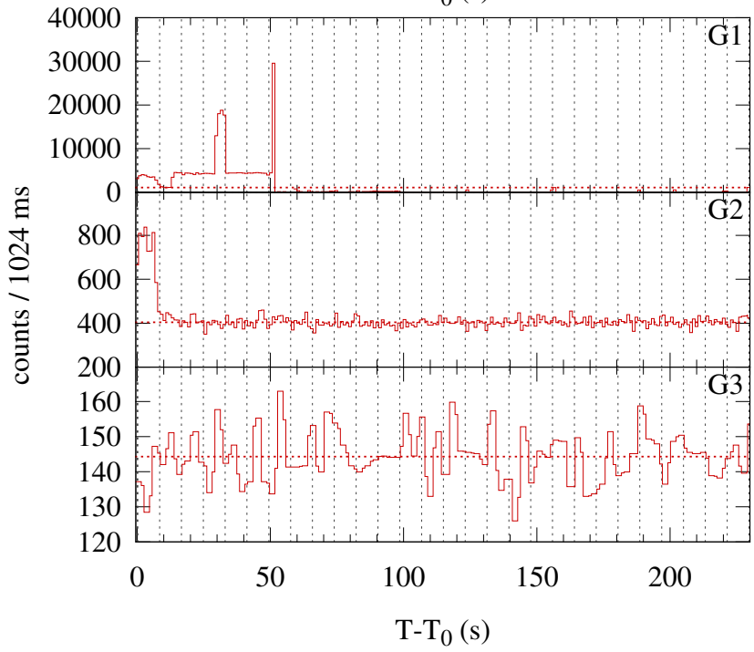
Konus-WIND S2 SOL2016-05-04T22:47 (C1.7) T 0 = 82051.631 s UT (22:47:31.631)
