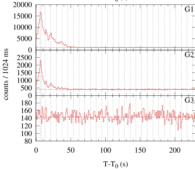
Konus-WIND S2 SOL2016-07-21T11:17 (C7.2) T_0 = 40667.664 s UT (11:17:47.664)
