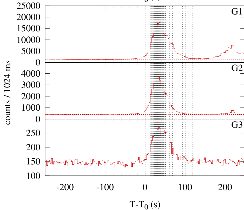
Konus-WIND S2 SOL2016-07-23T05:10 (M7.6) T_0 = 18600.810 s UT (05:10:00.810)
