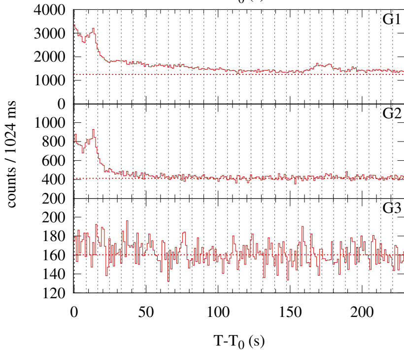
Konus-WIND S2 SOL2017-04-01T21:47 (M4.4) T_0 = 78459.65 s UT (21:47:39.65)
