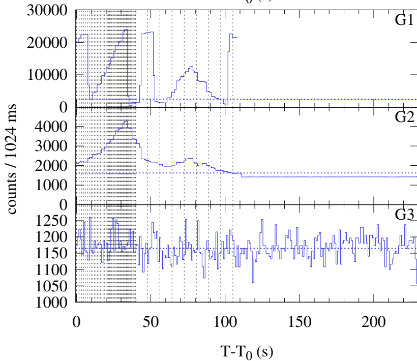
Konus-WIND S2 SOL2017-09-07T14:32 (X1.3) T_0 = 52345.599 s UT (14:32:25.599)
