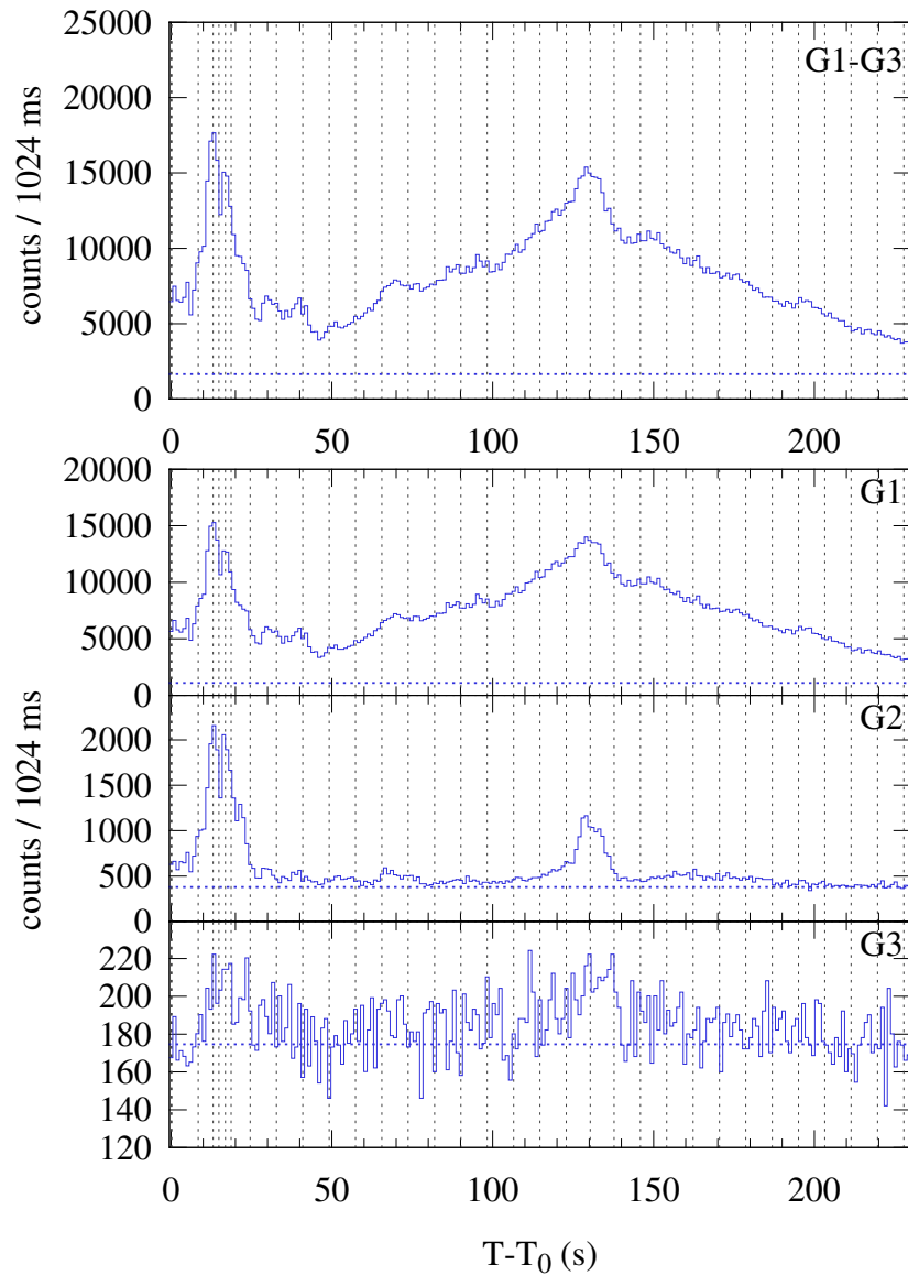
Konus-WIND S2 SOL2021-07-03T14:26 (X1.5) T_0 = 52000.472 s UT (14:26:40.472)
