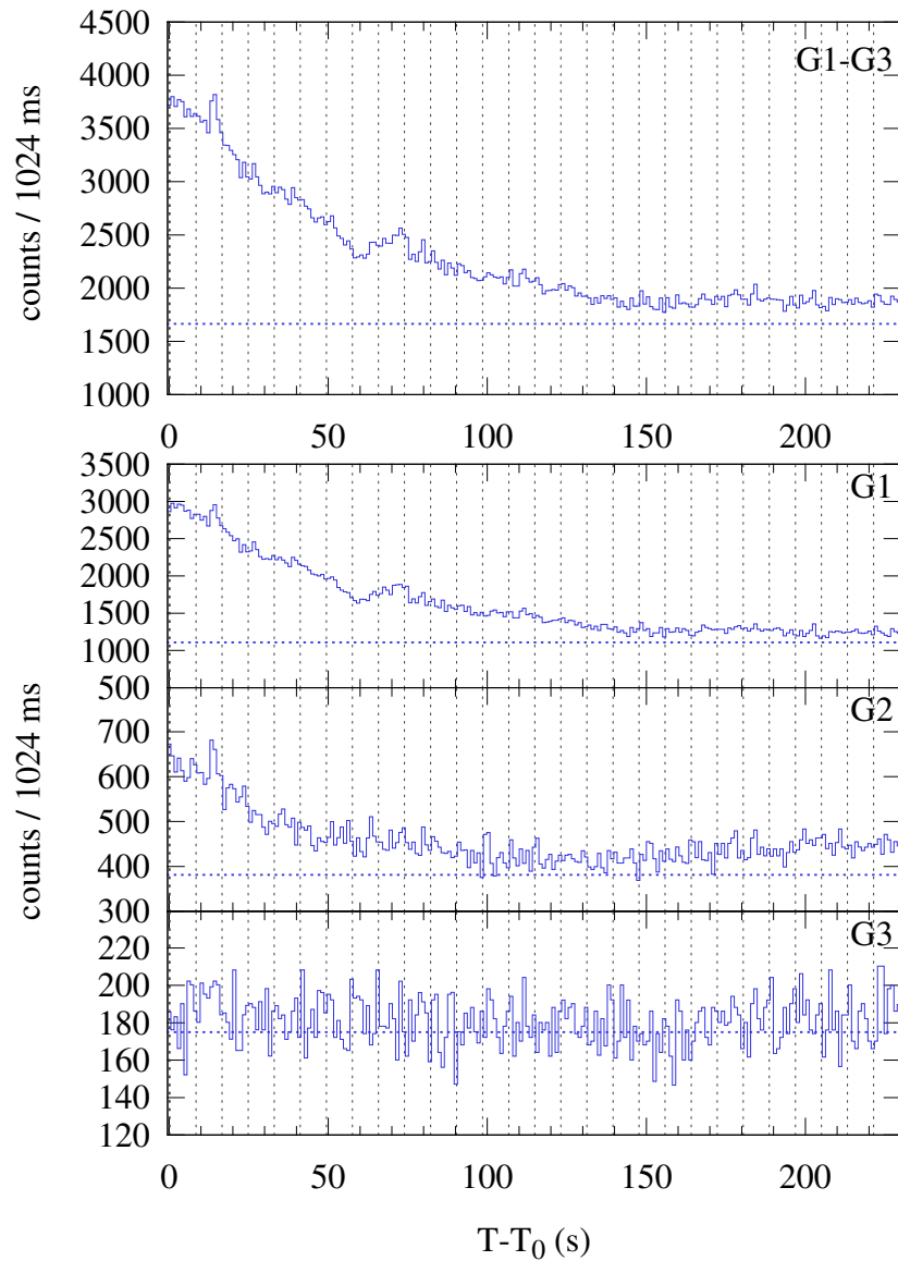
Konus-WIND S2 SOL2021-09-17T04:14 (C3.5) T_0 = 15257.27 s UT (04:14:17.27)
