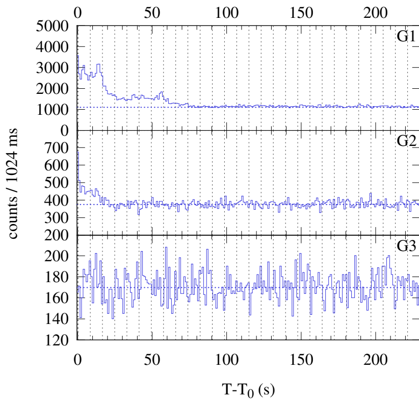
Konus-WIND S2 SOL2021-10-26T02:45 (M1.3) T 0 = 9939.970 s UT (02:45:39.970)
