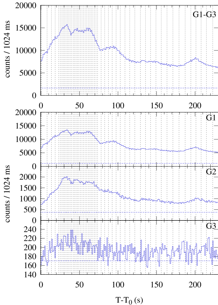
Konus-WIND S2 SOL2021-10-28T15:27 (X1.0) T_0 = 55646.140 s UT (15:27:26.140)
