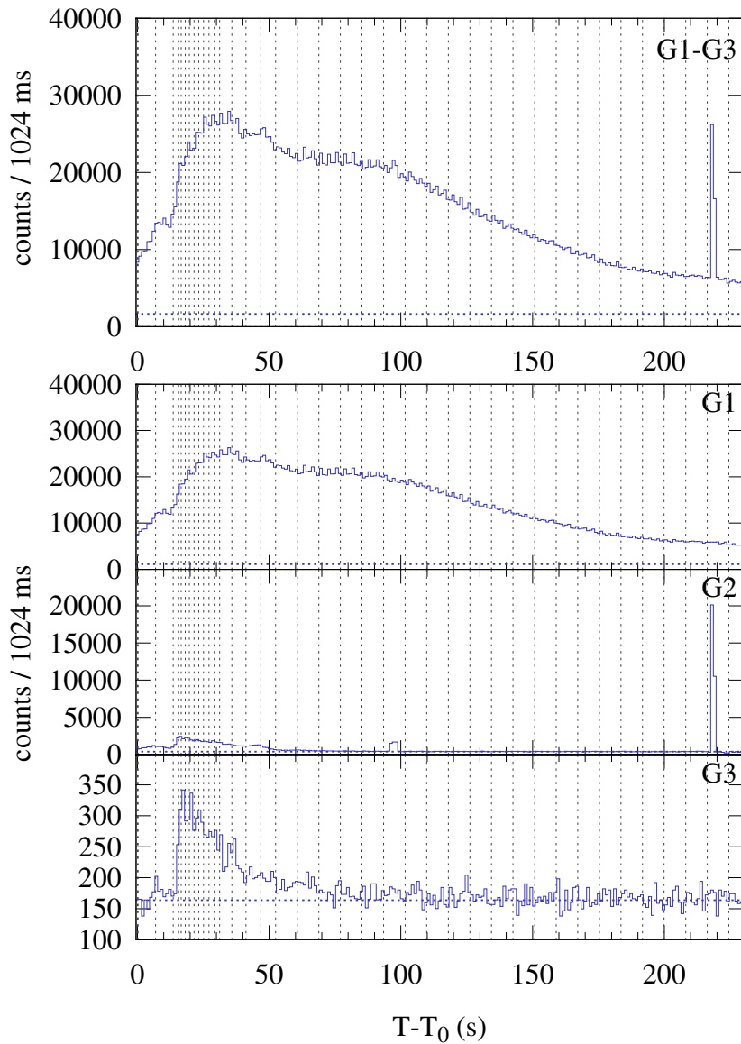
Konus-WIND S2 SOL2022-04-20T03:54 (X2.2) T_0 = 14070.711 s UT (03:54:30.711)
