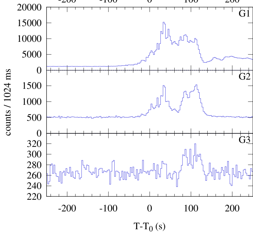
Konus-WIND S2 SOL2022-04-21T01:53 (M9.6) T_0 = 6826.253 s UT (01:53:46.253)
