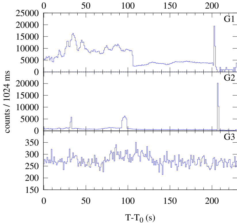
Konus-WIND S2 SOL2022-04-21T01:53 (M9.6) T_0 = 6826.253 s UT (01:53:46.253)
