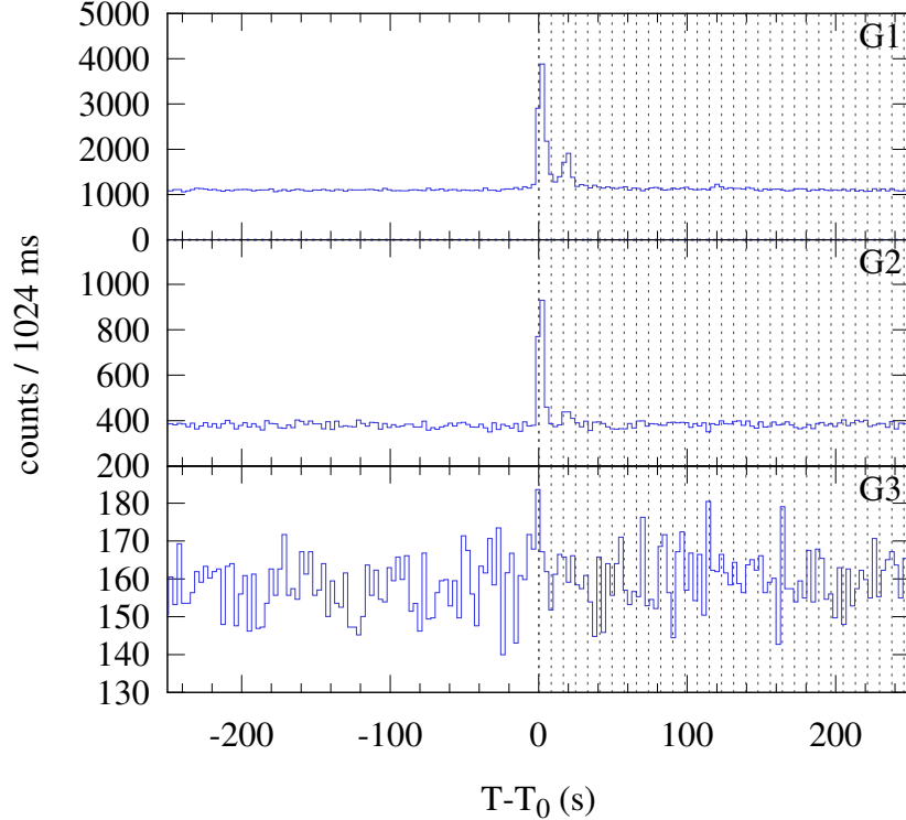
Konus-WIND S2 SOL2022-09-23T11:32 (C7.2) T_0 = 41540.130 s UT (11:32:20.130)
