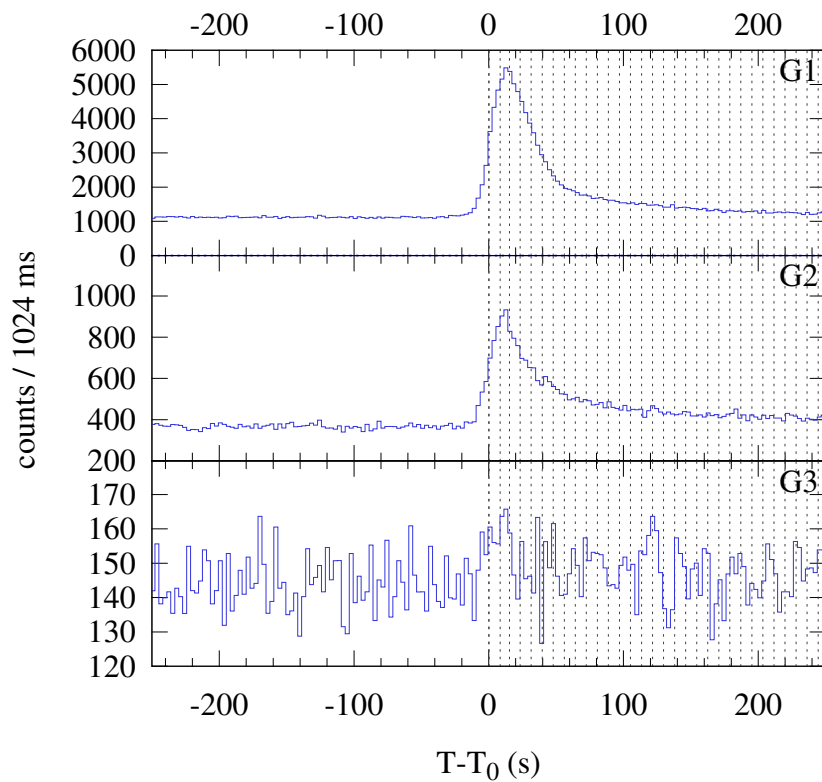
Konus-WIND S2 SOL2022-09-29T11:55 (C5.7) T_0 = 42904.71 s UT (11:55:04.71)
