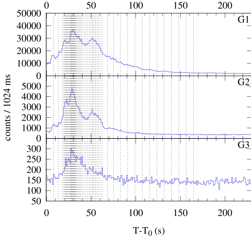
Konus-WIND S2 SOL2023-01-06T00:55 (X1.2) T_0 = 3314.287 s UT (00:55:14.287)
