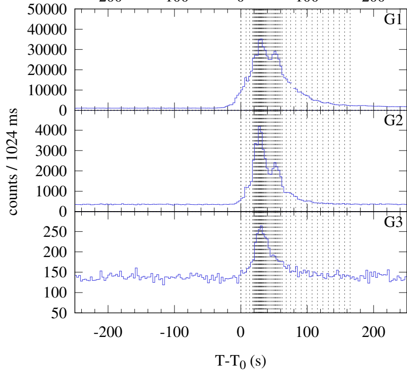
Konus-WIND S2 SOL2023-01-06T00:55 (X1.2) T_0 = 3314.287 s UT (00:55:14.287)
