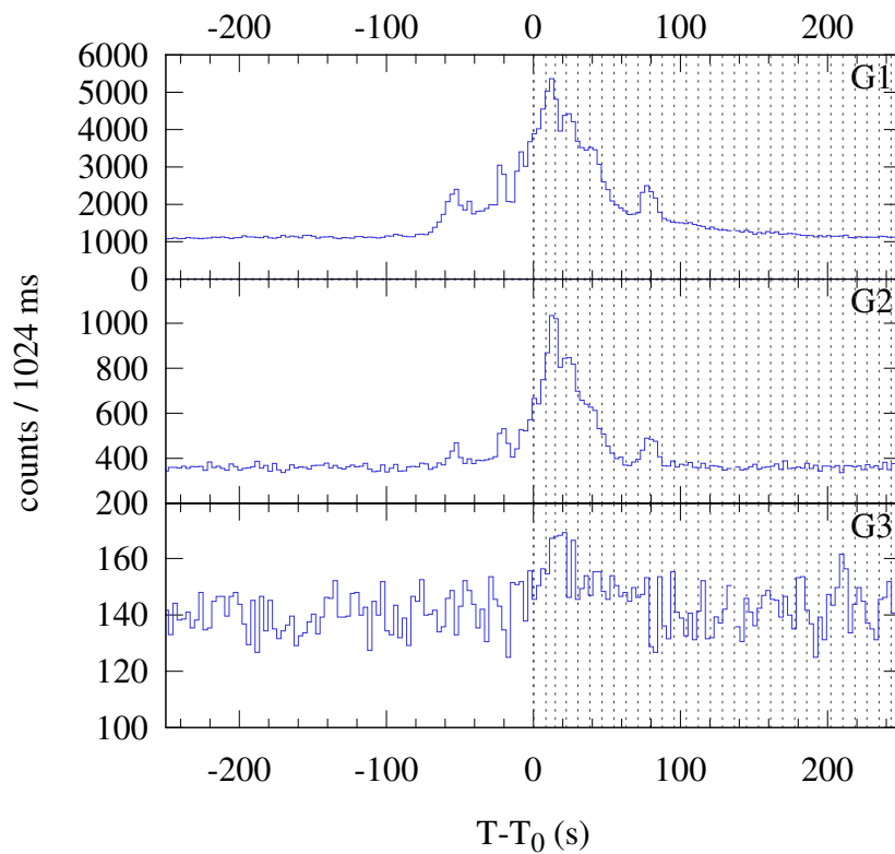
Konus-WIND S2 SOL2023-01-10T00:14 (M5.1) T_0 = 861.767 s UT (00:14:21.767)
