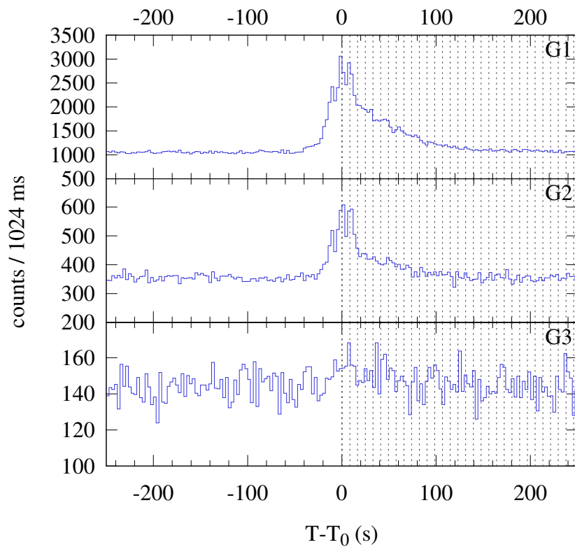
Konus-WIND S2 SOL2023-01-13T10:12 (M3.9) T_0 = 36764.322 s UT (10:12:44.322)
