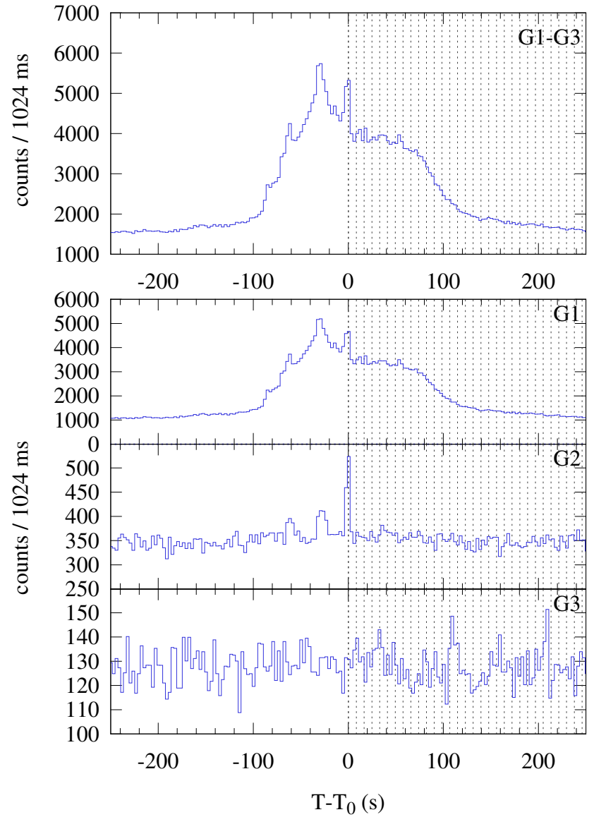
Konus-WIND S2 SOL2023-05-20T12:34 (M8.9) T_0 = 45270.987 s UT (12:34:30.987)
