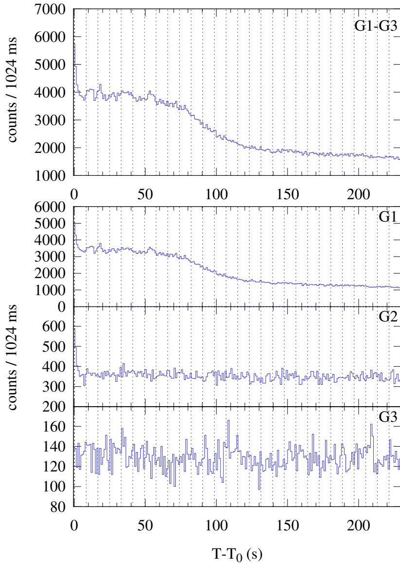
Konus-WIND S2 SOL2023-05-20T12:34 (M8.9) T_0 = 45270.987 s UT (12:34:30.987)
