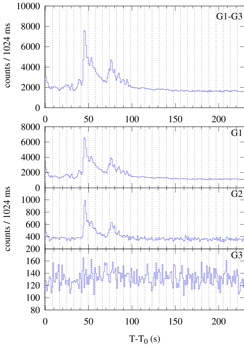
Konus-WIND S2 SOL2023-07-15T10:07 (M2.2) T_0 = 36455.716 s UT (10:07:35.716)
