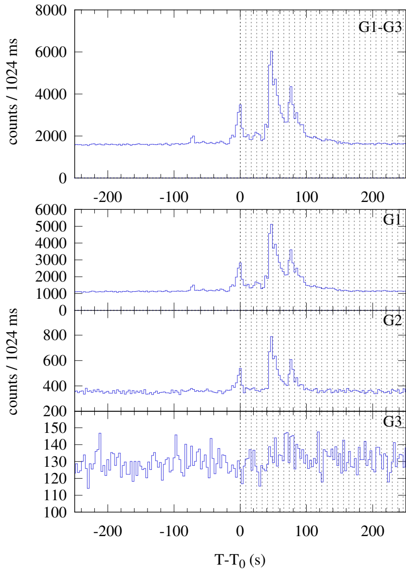
Konus-WIND S2 SOL2023-07-15T10:07 (M2.2) T_0 = 36455.716 s UT (10:07:35.716)
