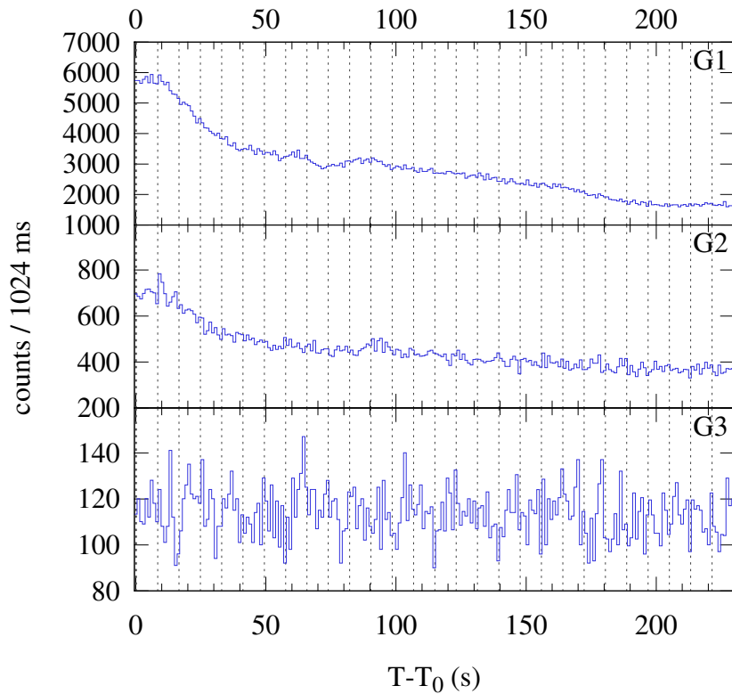
Konus-WIND S2 SOL2023-11-28T19:42 (M9.8) T_0 = 70965.465 s UT (19:42:45.465)
