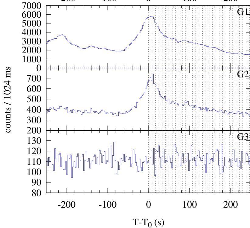
Konus-WIND S2 SOL2023-11-28T19:42 (M9.8) T_0 = 70965.465 s UT (19:42:45.465)
