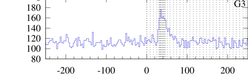
Konus-WIND S2 SOL2024-04-14T02:31 (M4.3) T_0 = 9061.77 s UT (02:31:01.77)
