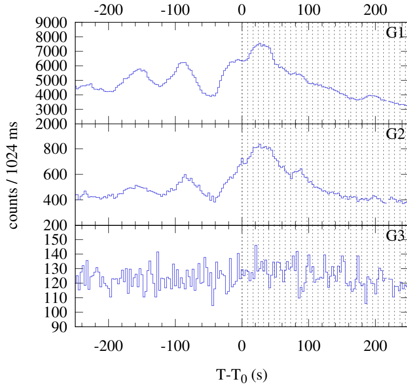
Konus-WIND S2 SOL2024-05-09T09:04 (X2.2) T_0 = 32654.784 s UT (09:04:14.784)
